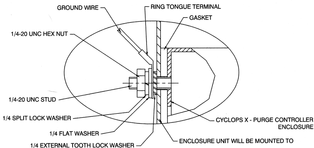
DETAIL OF GROUND CONNECTION
